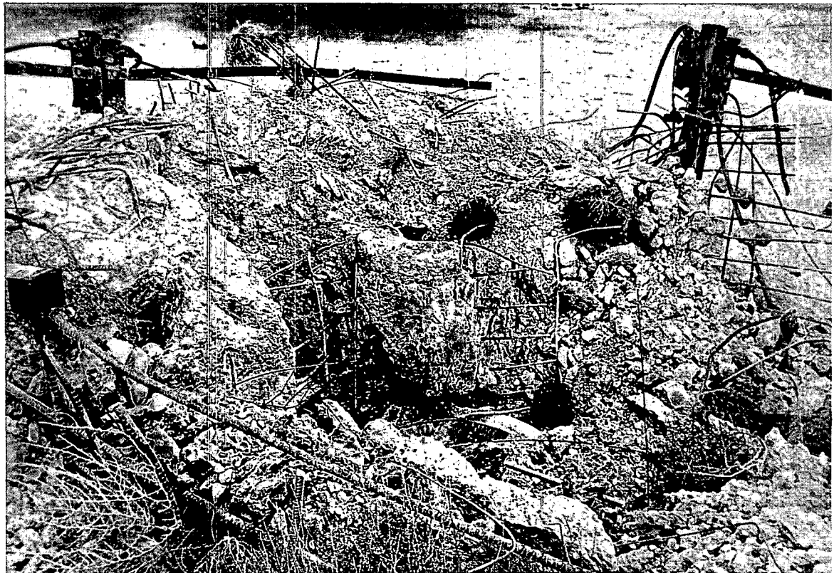
Fig. 7—Post-Quay event damage to tower base.
